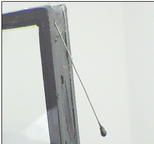
2. Apply a dab of silicone sealant at the end of the capillary tube after it has been cut.
