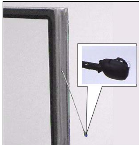
3. The IG unit must always be installed with the capillary tube pointing down along a vertical edge.
